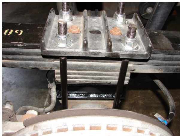
Fabricated Lift Blocks Installed and Secured
